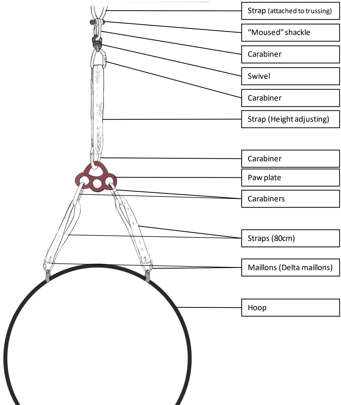
Rigging system
